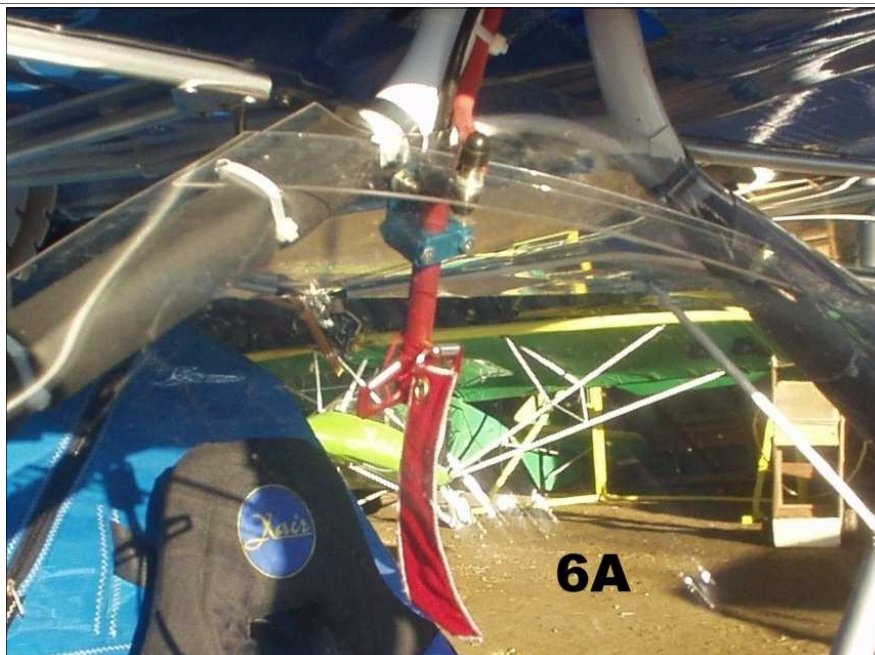
INSTALLATION OF USH PARACHUTE ON X-AIR MONTAGE PARACHUTE USH SUR X-AIR - 6
